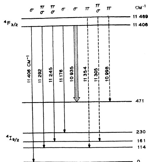
FIG. 4. Energy levels of {}^4F_{3/2} and {}^4I_{9/2} multiplets. The maser line terminates 471 \text{ cm}^{-1} above the ground state. Dashed lines indicate additional transitions seen at 77^\circ\text{K} .
