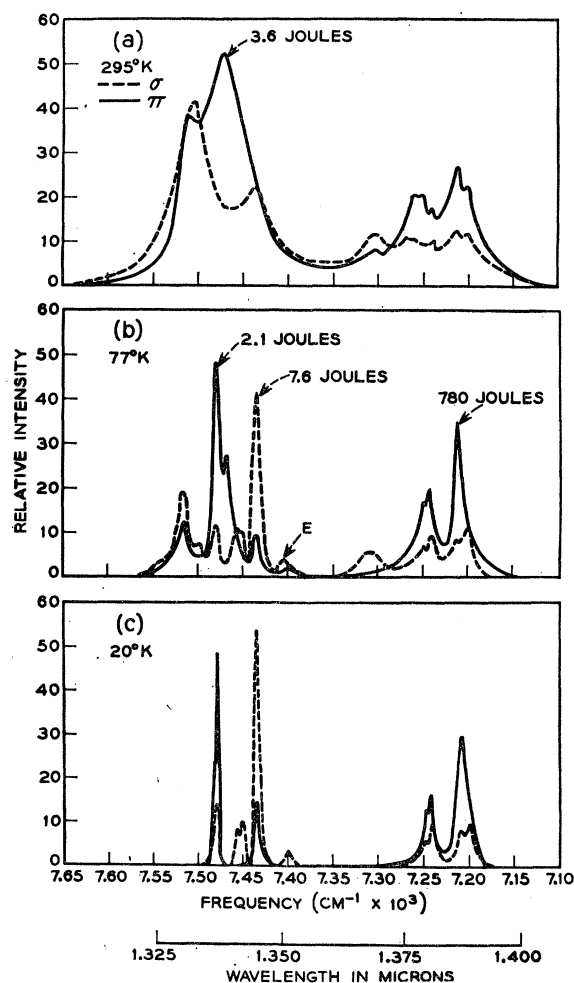
FIG. 1. Polarization of the {}^4F_{3/2} \rightarrow {}^4I_{13/2} emission in \text{CaWO}_4:\text{Nd}^{3+} ( \text{Na}^+ compensation) at 295, 77, and 20°K. Maser lines and threshold energies measured in an FT 524 xenon lamp are designated.
