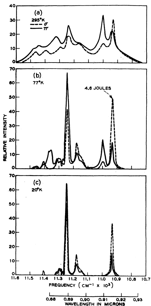
FIG. 3. Polarization of the {}^4F_{3/2} \rightarrow {}^4I_{9/2} emission in \text{CaWO}_4:\text{Nd}^{3+} ( \text{Na}^+ compensation) at 295, 77, and 20^\circ\text{K} . Maser oscillation is observed at 77^\circ\text{K} in the line at 0.9145\mu ( 10935 \text{ cm}^{-1} ).
