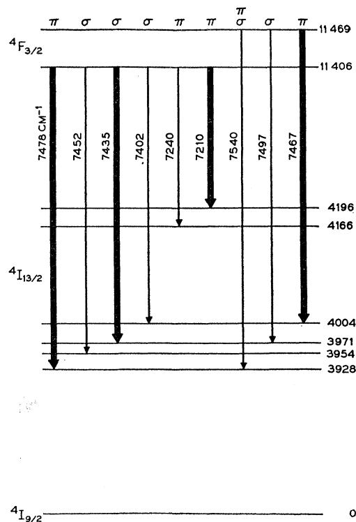
FIG. 2. Energy levels of {}^4F_{3/2} and {}^4I_{13/2} multiplets of \text{Nd}^{3+} in \text{CaWO}_4 ( \text{Na}^+ compensation). Maser transitions are indicated by heavy arrows.
